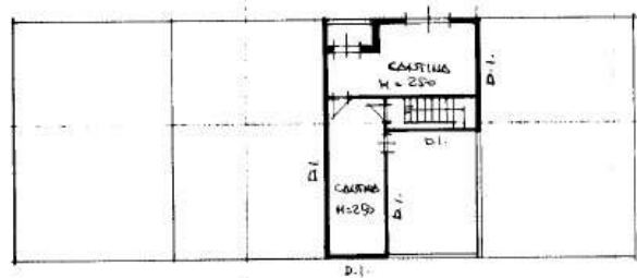
PIANO SEMINTERRATO
