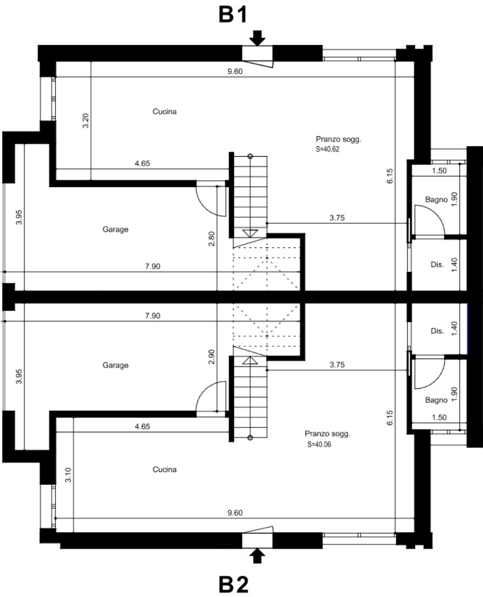
Piano Terra
