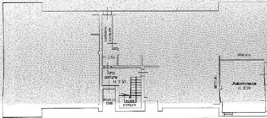
PIANO TERRA
